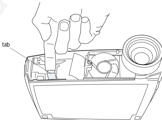
FIGURE 27 Pulling the tab on the lamp module
