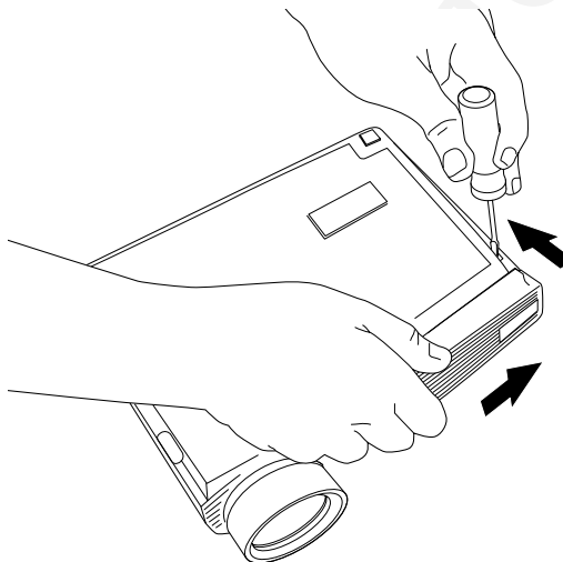
FIGURE 26 Disengaging and removing the lamp access grill
